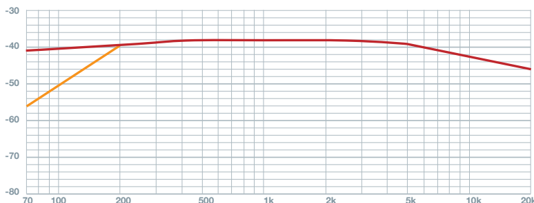
Frequency Response dB Ref 1V/Pa
